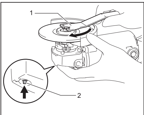
► 1. Lock nut wrench 2. Shaft lock
